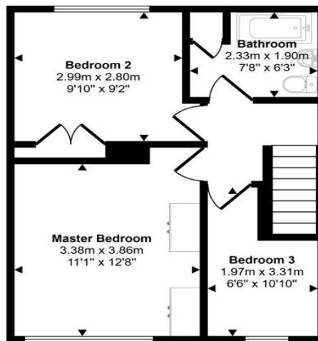
First Floor Approx 40 sq m / 426 sq ft
